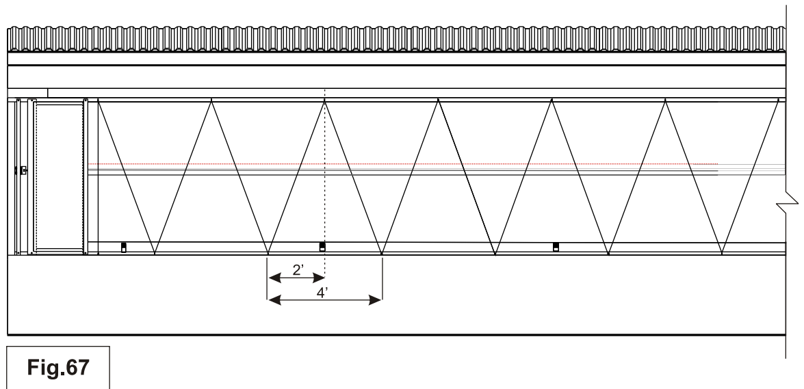
67. Wind rope:
